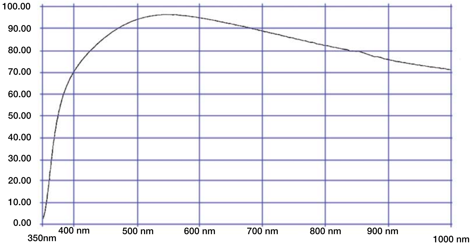
% Transmission Typical for EL1250B
